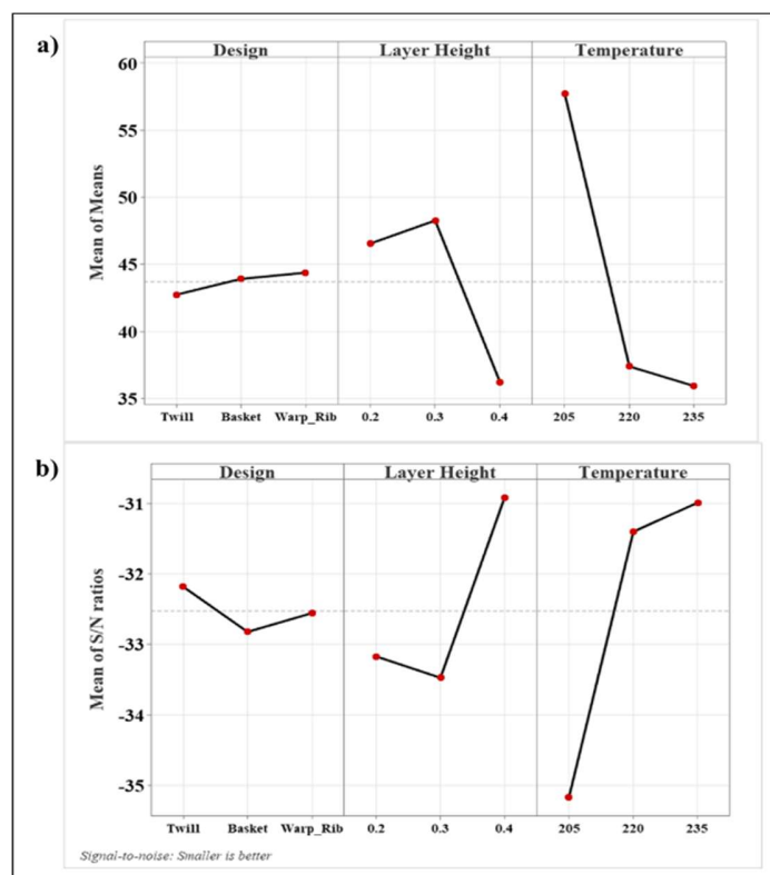
Fig. 11: Main effect plots for flexural modulus (MPa) of fabrics in warp direction: a) Mean of means b) Mean of S/N ratios
