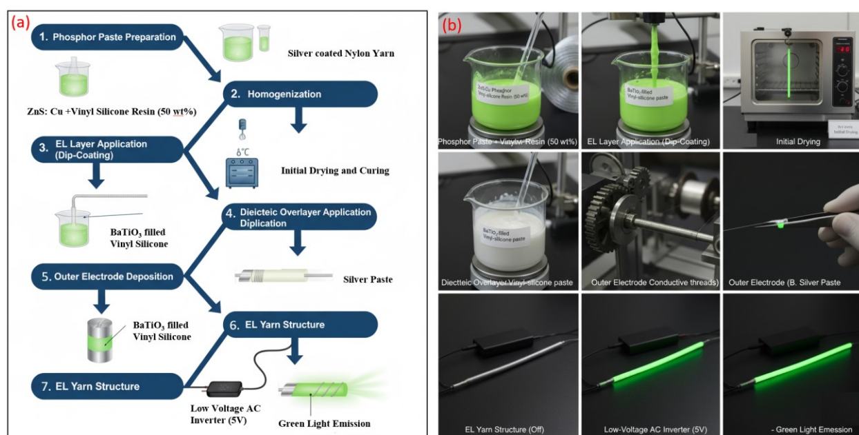
Figure 3. Composite paste preparation and Fabrication process and demonstration of electroluminescent (EL) yarn.
